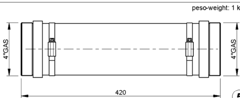
MANICOTTO FLESSIBILE FLEXIBLE HOSE tipo-type: FH15
