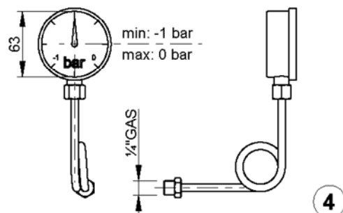
VACUOMETRO VACUUM GAUGE
